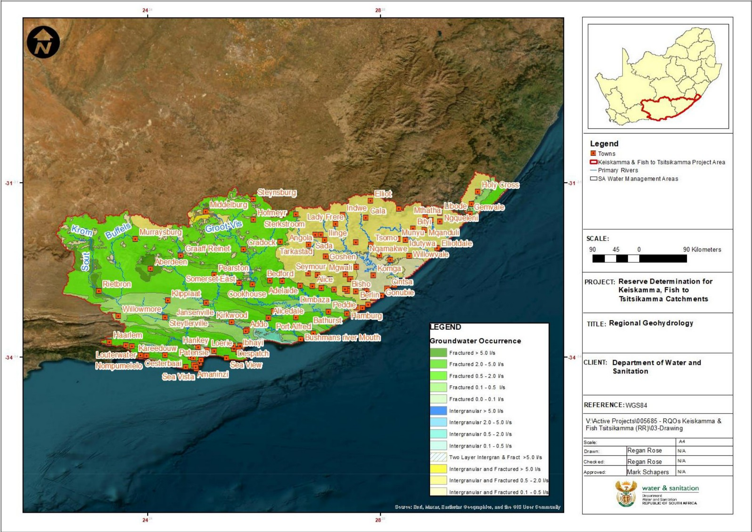
Figure 2: Regional Geohydrology
